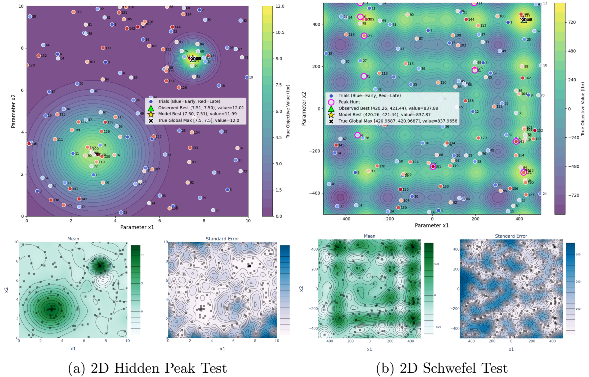
Figure 3: Two graphs demonstrating the results of 2-dimensional tests to validate the functionality of our ML model. Figure a shows the results for a hidden peak test while figure b does the same for a Schwefel function.
