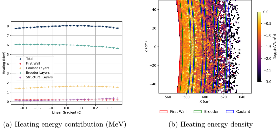
Figure 10: The heating energy (MeV) deposited in the blanket structures at values of \zeta is depicted in a. The heating energy density in a 2D slice of the breeder is shown in b.
