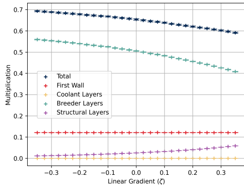
(a) Neutron multiplication
