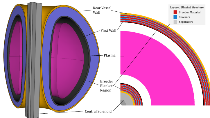
Figure 1: A pair of diagrams depicting the breeder dimensions and layered configuration. On the left, a 3D model shows the shape and arrangement of the overall structure. On the right a 2D slice demonstrates the layered formation of the heterogeneous blanket.
