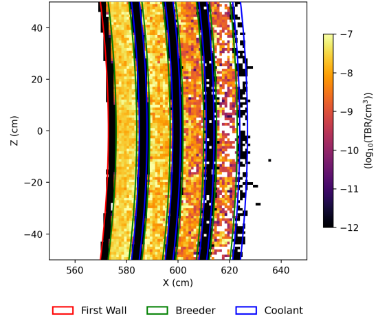
(b) Tritium breeding reaction Density
