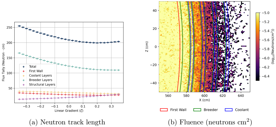
Figure 12: These figures demonstrate how neutron transport changes in the blanket. The effect of \zeta on the neutron track length measured by the ‘flux’ tally is shown in figure a. Figure b demonstrates the exponential decay of fluence throughout a 2D slice of the breeder.
