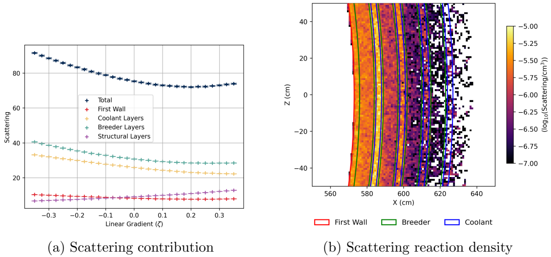
Figure 9: These figures demonstrate the change in scattering with values of \zeta (a) and the scattering density in a 2D slice (b).
