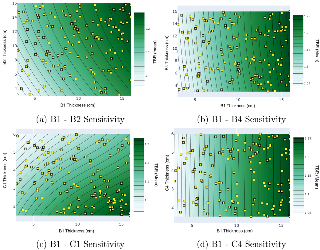
Figure 14: 2D projections of the sensitivity of TBR to the thicknesses of several blanket layers compared with the first breeder (B1).
