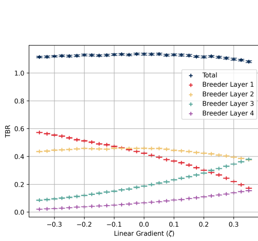
(a) Breeder TBR contribution
