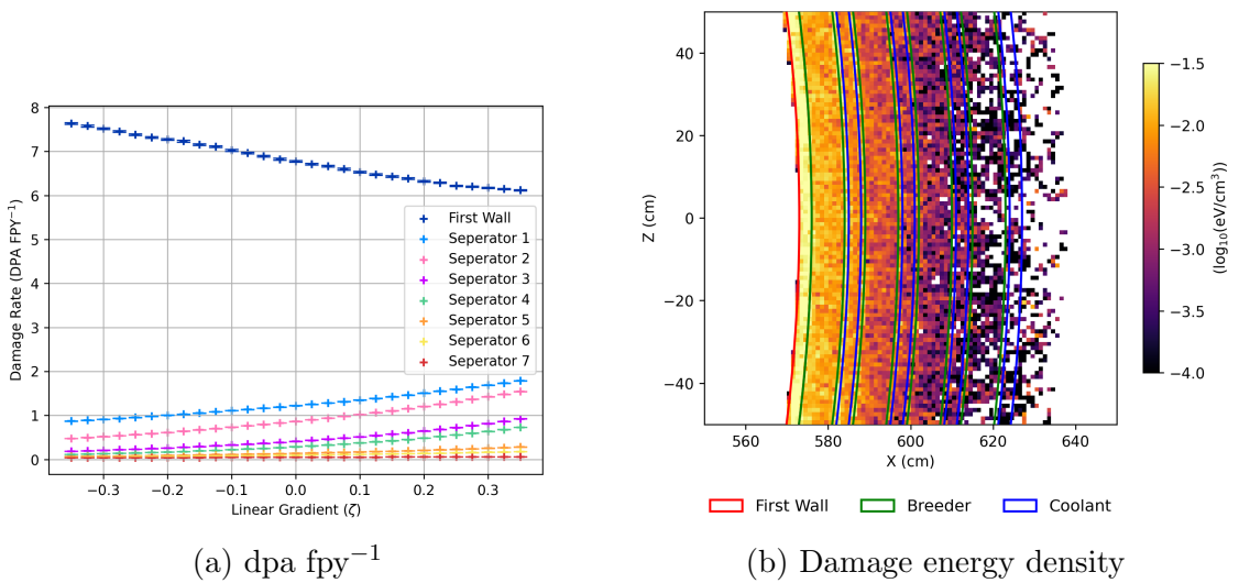
Figure 11: Figure a plots the dpa fpy -1 for a range of \zeta values while the damage energy deposited in the blanket regions is visualised in figure b.
