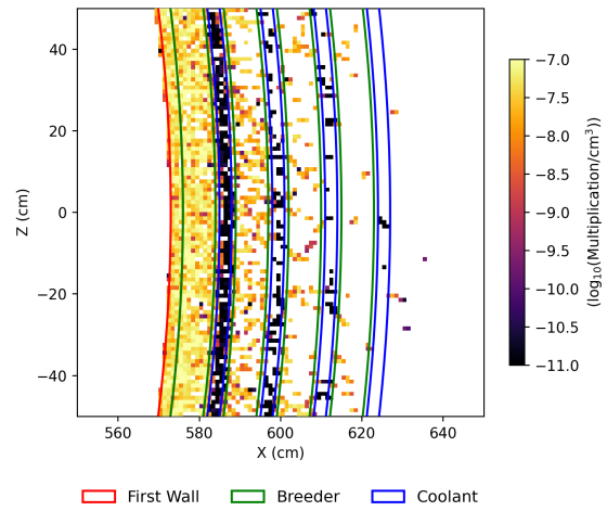
(b) Multiplication reaction density
